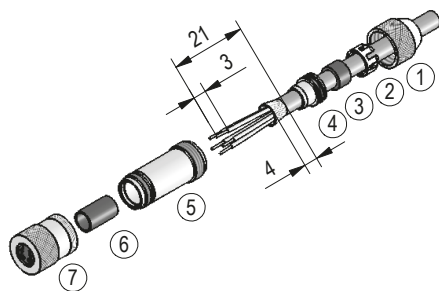
Fig. 6: Straight matting connector M8
