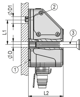
Fig. 1: Mounting dimensions
