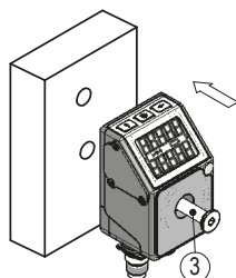
Fig. 2: Mounting
