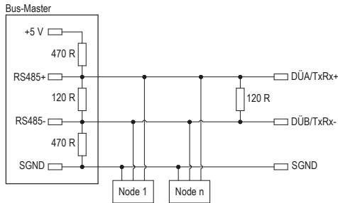
Fig. 3: Termination and level specification RS485
