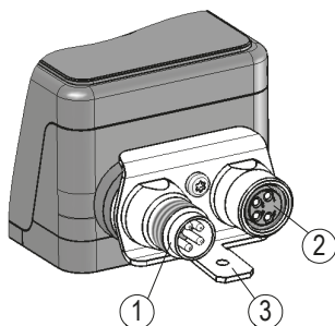
Fig. 4: Pin assignment
