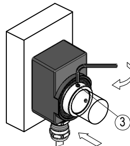
Fig. 3: Fastening torque for grub screw
