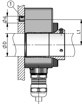
Fig. 1: Mounting dimensions
